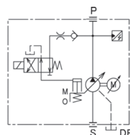
ASE10W&15W Dual Displacement Type
